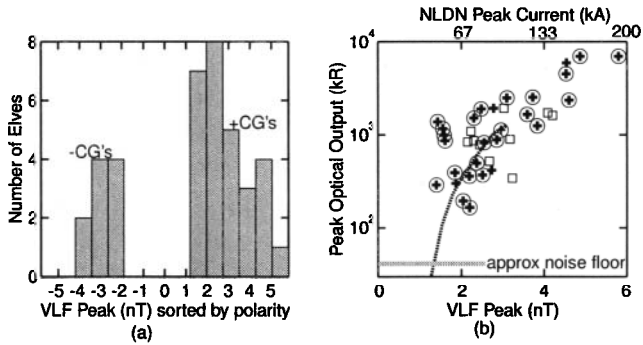
Figure 3. (a) Histogram of elves detected versus the strength of their causative VLF spheric, sorted by CG polarity. (b) Correlation between spheric strength (measured in equivalent wave magnetic field) and peak optical output. Squares and crosses show -CG and +CG events, respectively. A circle indicates that sprites were associated (within 100 ms) with the event. The dotted line shows the predicted relationship, scaled vertically to fit the observed intensities.
