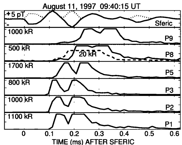
Figure 2. Photometer responses and simultaneous sferic recording for an unusually bright event, showing the photometric onset delay and the lateral 'expansion.' The unusually short onset delay for an event 571 km away is indicative of the low vertical extent of the flash. The dotted curve is the absolute value of the sferic, showing variations in optical output and causative EMP with similar time scales.
