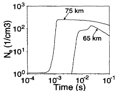
Fig. 4. The electron number density as a function of time at two selected altitudes—65 and 75 km.
