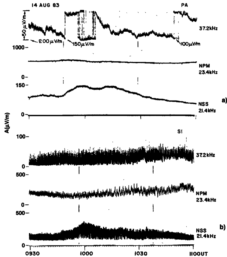
Figure 4. Comparison of Palmer and Siple analog charts during a 1 1/2-hour period when zigzag activity was detected at Siple and whistler-induced precipitation (Trimp events) occurred at Palmer. (a) Palmer records showing the amplitude of NPM, NSS, and a signal at 37.2 kHz from California. (b) Siple records for the same three signals (see map of Figure 2b).
