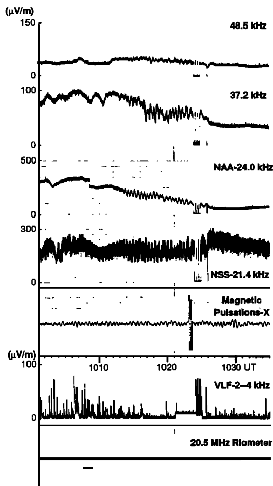
Figure 1. Section of an analog correlation chart from Siple Station, Antarctica, on August 25, 1986, showing a particularly clear example of simultaneous symmetrical zigzag activity beginning at \sim 1014 UT on multiple VLF/LF subionospherically propagating signals.
