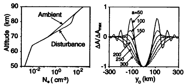
Figure 4. Right: Predicted change in the amplitude of the NAA-SD signal due to the appearance of a disturbance having a Gaussian shape ( e^{-(2r/a)^2} ) in the radial ( r ) direction, for different distance values of a , and as a function of the transverse distance y_0 between the center of the disturbance and the VLF path. Left: The ambient and disturbed ionospheric ionization profiles used in the model calculations.
