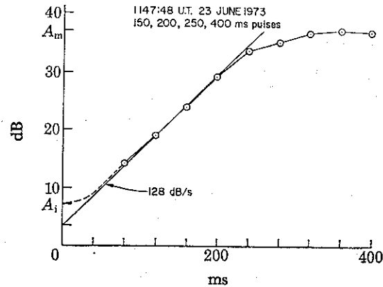
FIGURE 3. Average amplitudes of output pulses as a function of time after the start of the received pulse. Straight line fit gives exponential growth rate of 128 dB/s. Total growth is A_m - A_i = 30 dB. (From Helliwell & Katsufakis (1974).)
