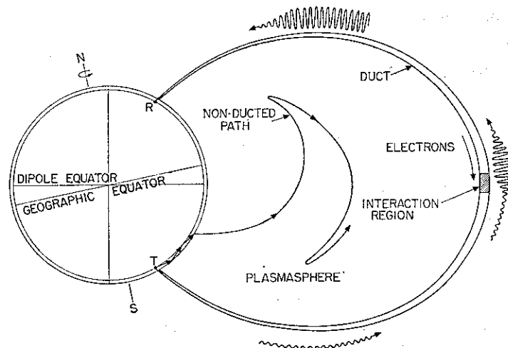
FIGURE 1. Sketch showing ducted and non-ducted whistler-mode paths in the magnetosphere. Three 0.5 s long ducted wave trains are shown before, during and after amplification on the equator. A group velocity of c/20 is assumed. Electrons precipitated by the ducted waves are absorbed in the shaded regions at the ends of the duct.
