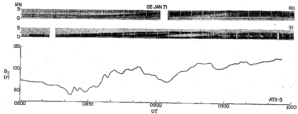
Fig. 7. Illustration of certain changes in center frequency of VLF noise during a substorm. The VLF records above, 0 to 5 kHz versus time, show data from the Roberval (RO)-Siple (SI) conjugate pair ( L \sim 4 ). The lower panel shows the magnetic B_z component from the ATS-5 GSFC magnetometer.
