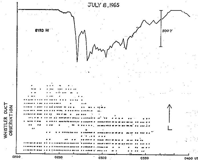
Fig. 5. Example of the apparent 'erosion' of whistler ducts observed from Eights Station during a substorm. Above is a transcription of the Byrd, Antarctica magnetic H component. Dots show the presence of individual whistler traces observed at Eights, Antarctica. The L coordinate is not shown explicitly, but L increases upward.
