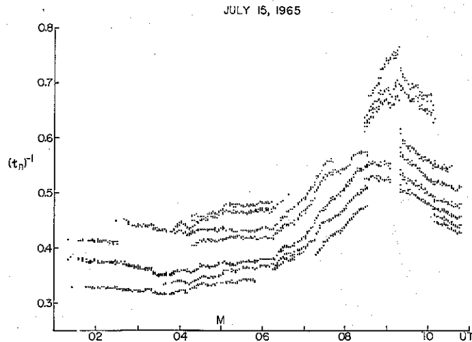
Fig. 2. Graph of the reciprocal of whistler travel time at the nose ( \tau_n^{-1} ) vs. time, illustrating convection activity on several whistler paths over a 10-hour period on July 15, 1965 that included an isolated substorm. Local midnight at the observing whistler station (Eights, Antarctica) is indicated by M. The data gap near 0910 UT is due to a magnetic recording-tape change during a period of increased difficulty in determining continuity of whistler paths (from CARPENTER et al. , 1972).
