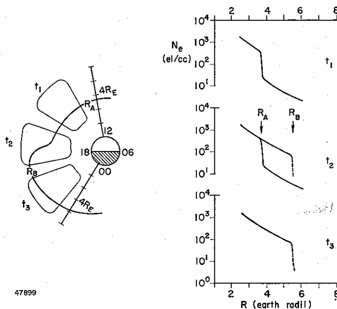
47899 Fig. 6. Diagram of the method by which the viewing area of a single station is used to detect the presence of the dusk-side bulge in the plasmasphere. The equatorial viewing area of the ground station is shown at three successive times, t_1 , t_2 and t_3 . The corresponding equatorial profiles deduced from the data (without considering longitudinal spread of the paths) are shown at the right (from CARPENTER, 1970).
