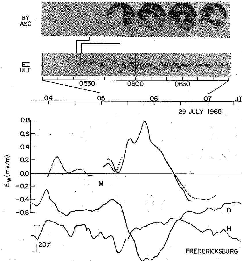
Fig. 4. A substorm event showing the near simultaneity of an auroral expansion, a Pi 2 micropulsation event, a rapid increase in westward electric field in the outer plasmasphere, and a westward turning of the magnetic D component at a midlatitude observatory (from CARPENTER and AKASOFU, 1972).
