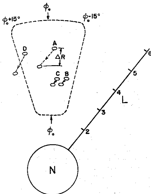
Fig. 1. Diagram of the whistler method of tracking the cross- L motions of whistler ducts. The dashed curve outlines the approximate equatorial region that a ground station at longitude \phi_0 and L \sim 4 is capable of observing, given the presence of suitable lightning source activity in the conjugate region. The equatorial positions of four representative whistler ducts are labeled A, B, C and D. In general the ducts are in motion with respect to the viewing area. The radial component of this motion may be relatively accurately determined by present techniques (from CARPENTER et al., 1972).
